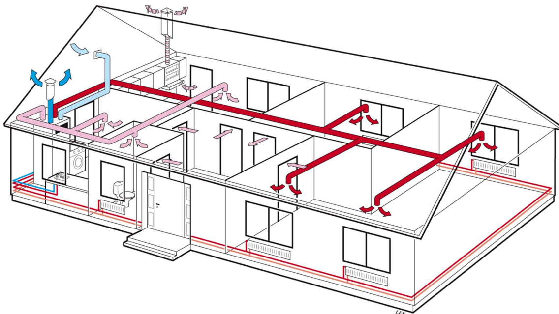
EAHP with supply and exhaust ducting - type 2
