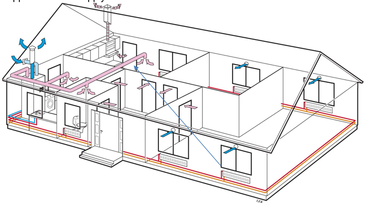
EAHP with Inlet only ducting – type 1
