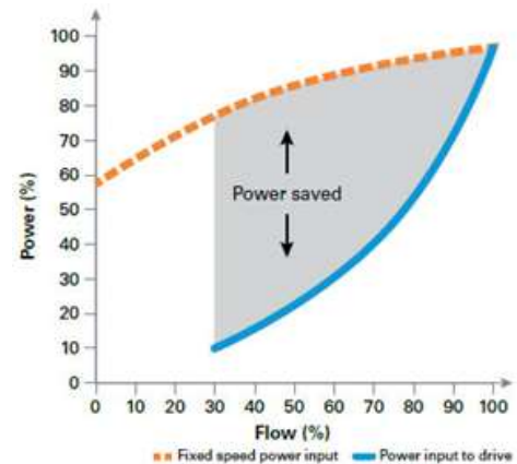
Power savings of Variable speed drive over fixed speed pumps
